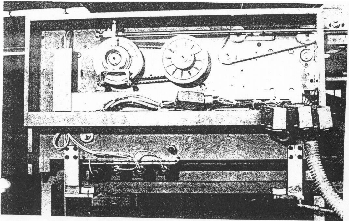
80 372 Laufrolle 7973 Kurvenrolle
